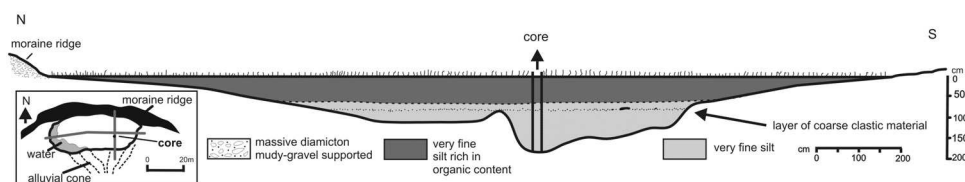
Fig. 3. Plan and cross section of the peat bog from the Pysznińska glade with the location of sediments core
