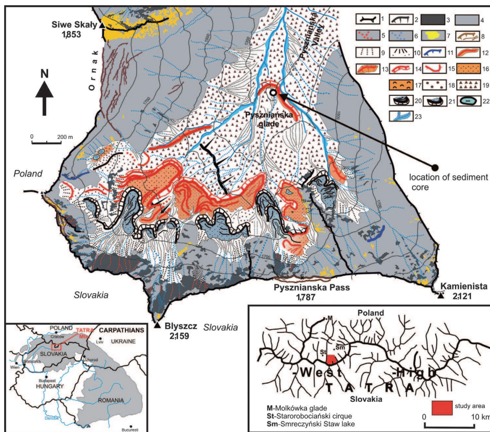
Fig. 1. Geomorphological map of the upper part of the Pyszniańska Valley (according to P. Kłapyta), 1 — crest, 2 — structural threshold, 3 — rocky slopes and rockwalls, 4 — debris mantled slopes, 5 — chutes, 6 — gullies, 7 — periglacial debris covers, 8 — system of fissures and sacking scarps, 9 — rockfall talus, 10 — alluvial cone, 11 — glacial cirque edge, 12 — symmetrical moraine ridge, 13 — asymmetrical moraine ridge, 14 — massive fronts moraines, 15 — protalus ramparts, 16 — ablation moraine covers (blocky type), 17 — ablation moraine covers (hummocky moraine), 18 — weathered, discontinuous moraine covers, 19 — ground moraine covers, 20 — relict rock glaciers, 21 — protalus bulges, 22 — dead-ice depression, 23 — stream channels
